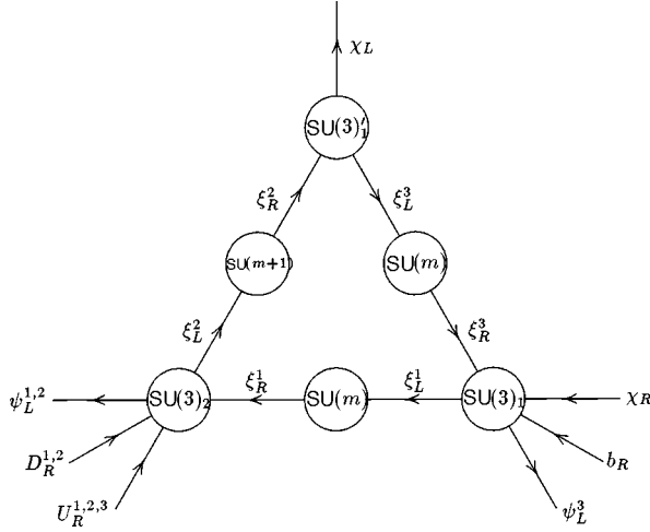
FIG. 3. Chivukula, Dobrescu, Georgi, and Hill's top-color model [10]. The low energy effective theory for this model contains a single composite Higgs doublet.
