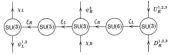
FIG. 2. Another top-color theory constructed so that \bar{\chi}_L t_R and \bar{\chi}_R \chi_L terms are forbidden at tree level. Instead, these terms arise dynamically in the low energy theory.
