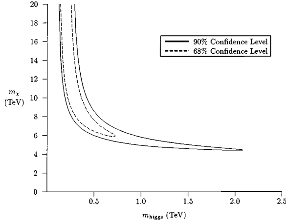
FIG. 7. The allowed set of m_\chi and m_{\text{Higgs}} masses based on current precision electroweak tests.
