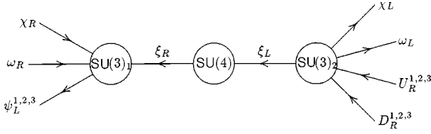
FIG. 1. An example of a simple model that can realize a top-color seesaw. The central gauge group is chosen so that the theory is free of anomalies.
