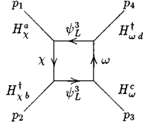
FIG. 8. This graph produces the leading matching contribution to the custodial SU(2)-violating operator O_4^{\chi\omega} .
