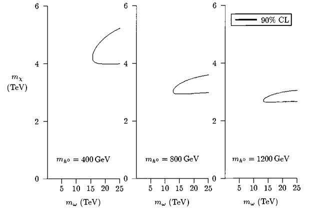
FIG. 12. This figure shows the regions in the \chi - \omega mass plane allowed by the current precision electroweak experiments when the massive Higgs fields, h^0 , H^0 , and H^\pm , have a common mass of 400, 800, and 1200 GeV, respectively. In each of these plots, the light pseudoscalar Higgs field, A^0 , was given a mass of 100 GeV.
