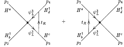
FIG. 6. These graphs give the leading running contribution to the operator in the low energy theory that violates custodial SU(2).
