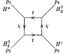
FIG. 5. This diagram gives the leading matching contribution to the operator that violates custodial SU(2) in the effective theory for energies below the \chi mass.
