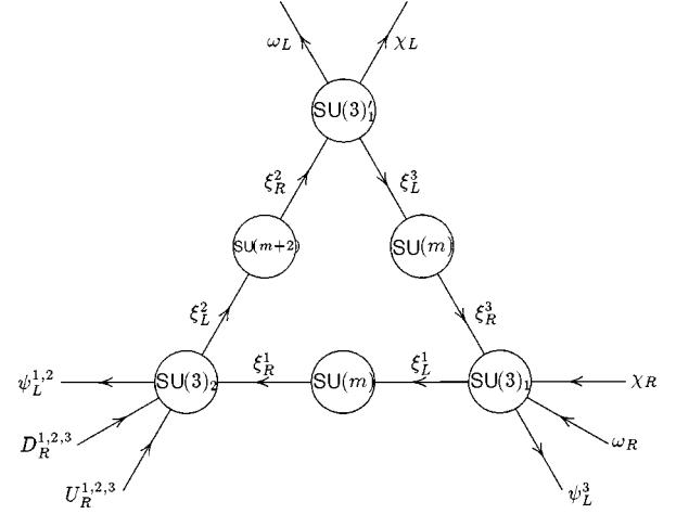
FIG. 4. Another top-color model which contains two composite Higgs doublets in the low energy effective theory.
